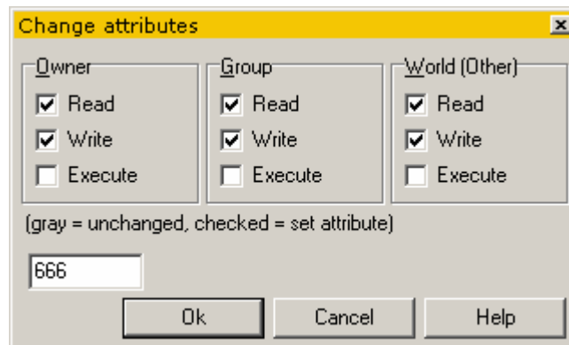
Pic. 2. Permission settings for the directory
