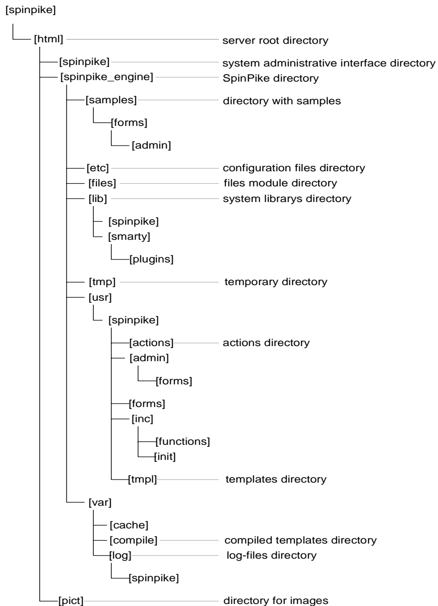
Pic. 1. SpinPike™ directories structure
